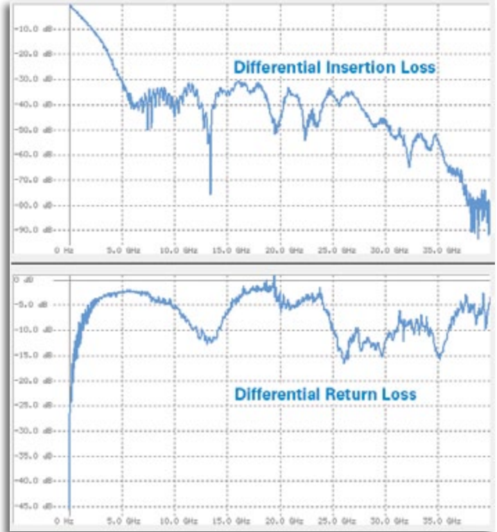
SPARQ mixed-mode measurements are useful for determining the quality of high-speed channels.
