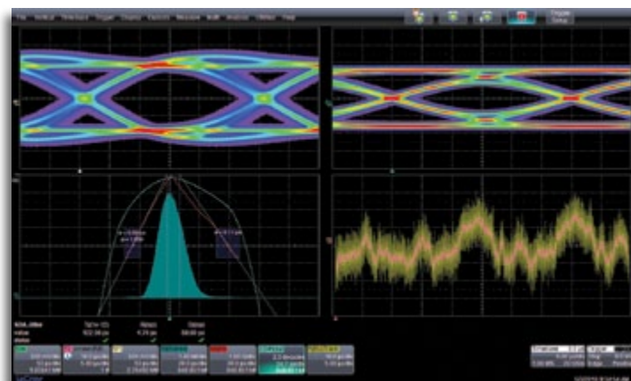
SPARQ produced S-parameters are shown here working with LeCroy oscilloscope based tools like the popular serial data analysis (SDA) and Eye Doctor™ tools in a co-simulation environment to predict the behavior and equalization requirements of a high-speed serial channel.
