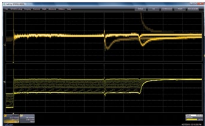
Raw TDR mode persistence showing added near- and far-end capacitance (upper grid) and the effect of wiggling a bad cable (lower grid).
