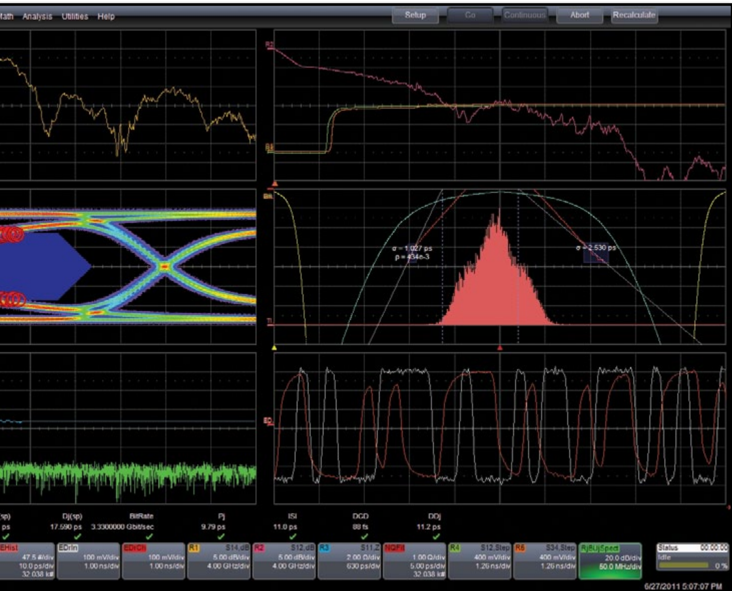
Signal Integrity Studio enhances the modeling and simulation capabilities of the LeCroy SPARQ application, adding eye and jitter measurements.
